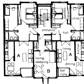
4 Three dwellings per floor: 2 apartments and one studio flat
